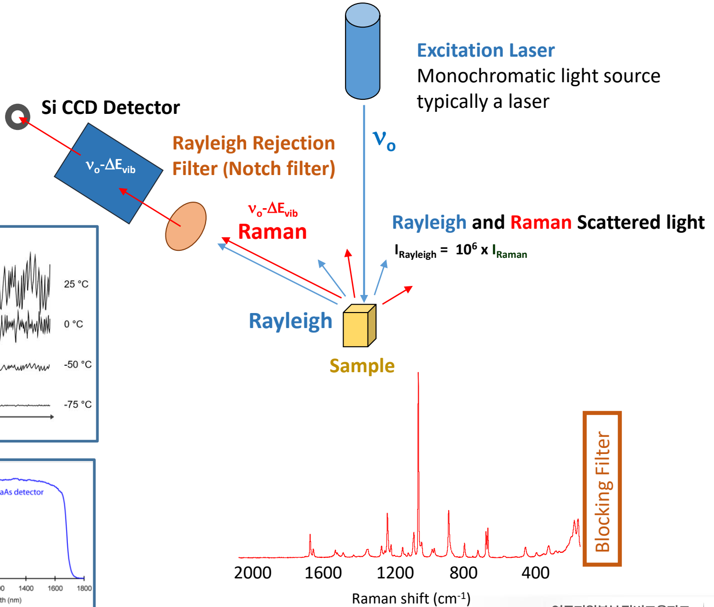
Grating spectrometer
